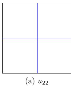
Figure 13.4: \lambda = 8
