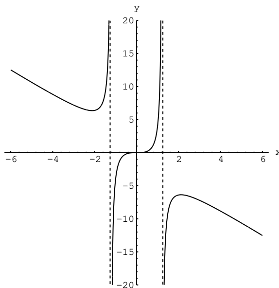
Figure 2.2: y(x) which solves xy' = 3y + y^2/x with y(1) = 4 .
