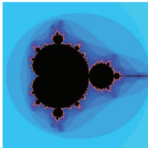
Figure 9.16: Mandelbrot set. Black regions stay bounded; colored regions become unbounded with shade indicating how rapidly the system becomes unbounded. Image generated from https://cs.clarku.edu/~djoyce/julia/explorer.html .
