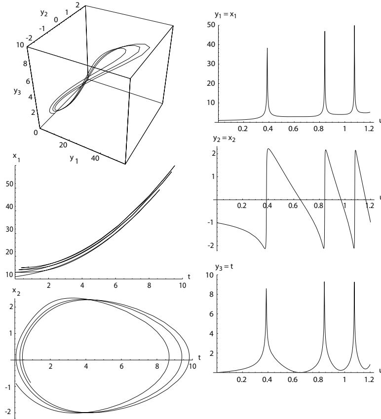
Figure 9.3: Solutions for one set of initial conditions, y_1(0) = 1, y_2(0) = -1, y_3(0) = 0 , for second paradigm example: trajectory in phase volume (y_1, y_2, y_3) ; also y_1(u), y_2(u), y_3(u) and x_1(t), x_2(t) . Here y_1 = x_1, y_2 = x_2, y_3 = t .
