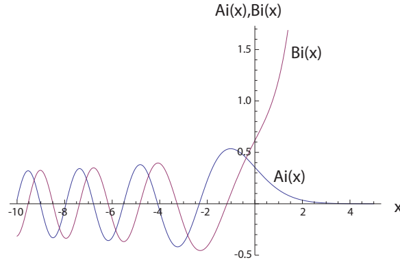
Figure 10.8: Airy functions \text{Ai}(x) and \text{Bi}(x) .
