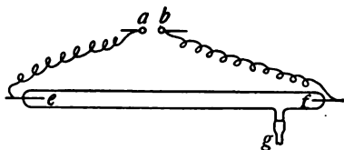
FIG. 418.—An Aurora tube.
