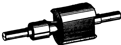
FIG. 282.—A shuttle armature.
