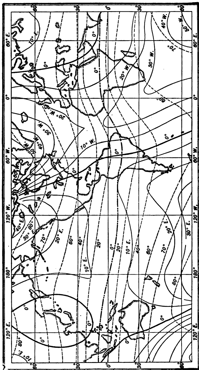
Fig. 184.—Magnetic map of the earth for 1910. Isogonic lines ———. Isoclinic lines ..... .
