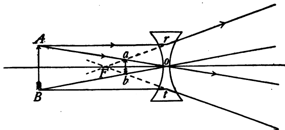
FIG. 385.—Construction of a virtual image by a concave lens.
