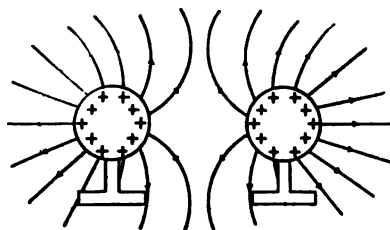
FIG. 195.—Electric field between like charges.
