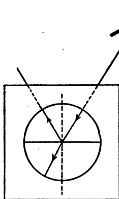
FIG. 367.—Part of the ray is reflected and part passes into the water and is refracted.
