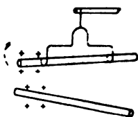
FIG. 186.—Repulsion of like charges.
