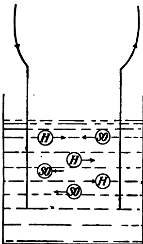
FIG. 262.—The current is carried through the solution by ions.
