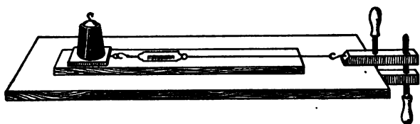
FIG. 111.—A method for testing the friction between surfaces.
