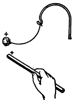
FIG. 190.—The pith ball charged by contact is repelled.
