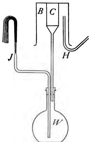
FIG. 7.—Effusion of gases.
