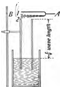
FIG. 328.—Explanation of resonance.
