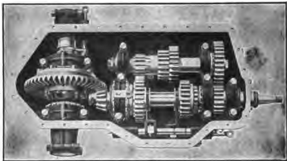
FIG. 94.—Transmission gear of an automobile.
