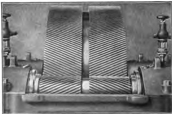
FIG. 95.—Reducing gear of a steam turbine.
