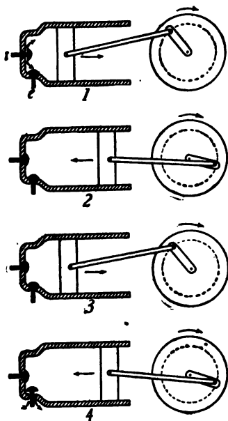
FIG. 165.—The four cycles of a gas engine.
