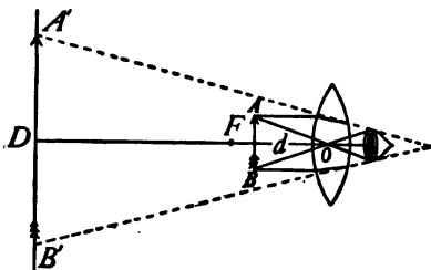
FIG. 388.—Action of the simple microscope.
