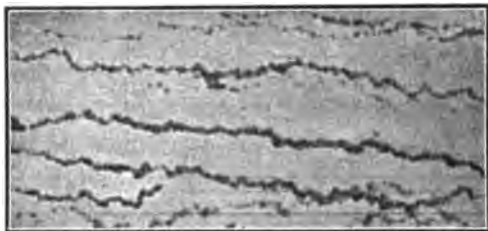
FIG. 417.—Photograph of Brownian movement. This record is prepared by the aid of Siedentopf's ultra-microscope and a plate moving uniformly across the field from left to right.
