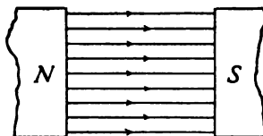
FIG. 296.—The magnetic field between two unlike poles.
