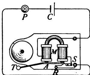
FIG. 241.—An electric bell and its circuit.
