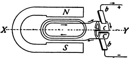
FIG. 292.—The armature coils are connected to a commutator producing a direct current.
