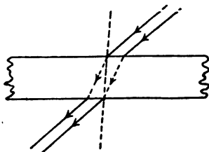
FIG. 368.—Illustrating the laws of refraction of light.
