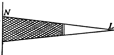
FIG. 346.—Shadow from a small source of light.
