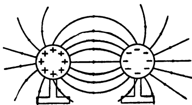
FIG. 194.—Electric field between unlike charges.
