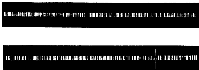
FIG. 408.—The bright line spectrum of iron and its coincidences with some of the dark lines of the solar spectrum.
