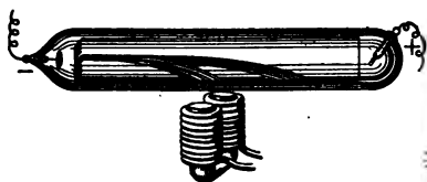
FIG. 421.—The stream of cathode rays is deflected by a magnet.
