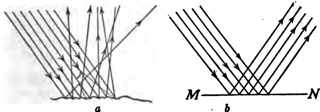
FIG. 353.—Reflection of light, (a) diffused, (b) regular.
