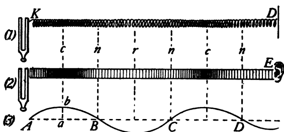
FIG. 318.—Longitudinal waves (1) in a spring, (2) in air, and (3) graphic representation.
