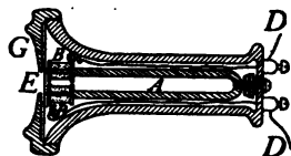
FIG. 310.—A telephone receiver. This receiver has a permanent horseshoe magnet with a coil about each pole.
