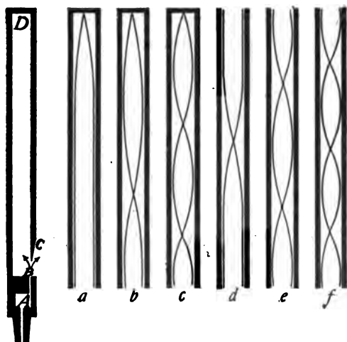
FIG. 341.—(R) Cross section of an organ pipe showing action of tongue at C. (a) The fundamental tone has a wave length four times the length of closed tube; (b) and (c) how the first and second overtones are formed in a closed pipe; (d) the fundamental tone of an open pipe is one-half the wave length; (e) and (f) first and second overtones of open pipe.
