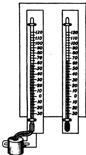
FIG. 149.—Wet and dry bulb hygrometer.
