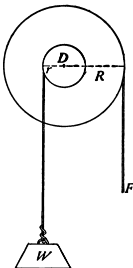
FIG. 93.—The wheel and axle considered as a lever of the first class.
