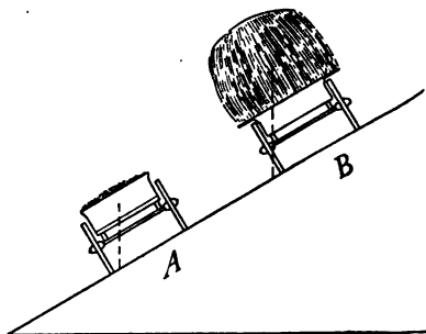
FIG. 77.— B will overturn; A will not.
