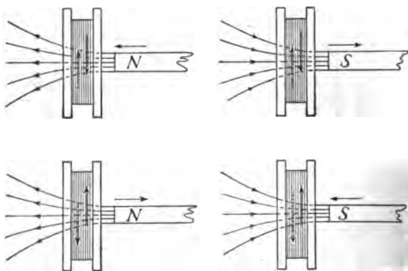
FIG. 283.—The induced current has a field which opposes the motion of the magnet.
