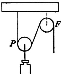
FIG. 96.—A single movable pulley.
