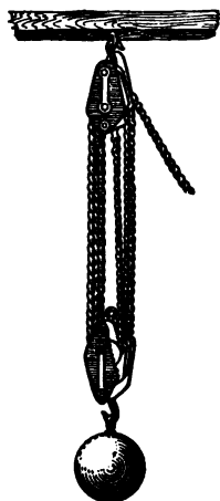
FIG. 97.—Block and tackle.
