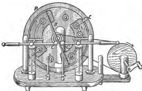
FIG. 214.—The Toepler-Holtz induction machine.
