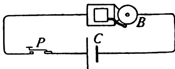
FIG. 218.—Diagram of an electric bell circuit.
