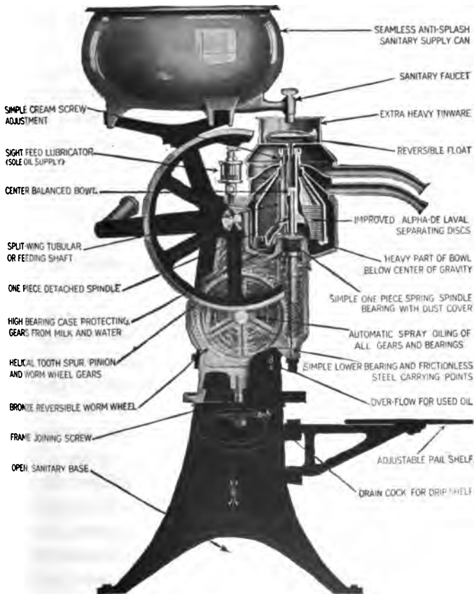
FIG. 60.—Cross-section of the DeLaval cream separator.
