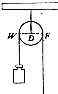
FIG. 98.—The fixed pulley considered as a lever of the first class.
