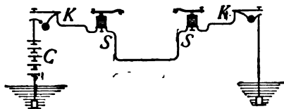
FIG. 237.—A simple telegraph circuit.
