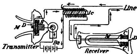
FIG. 312.—Telephone instruments at one end of a talking circuit.
