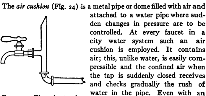
FIG. 24.—The short pipe above the faucet contains air forming an air cushion.
