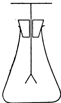
FIG. 187.—An aluminum foil electroscope.
