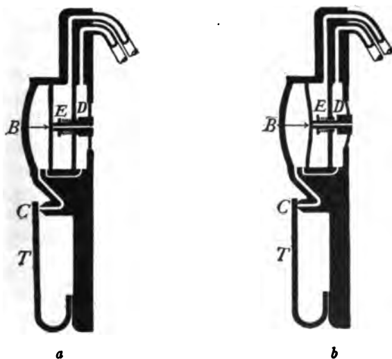
FIG. 148.—A thermostat. (Johnson System.)
