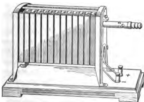
FIG. 122.—A thermo-electric generator.
