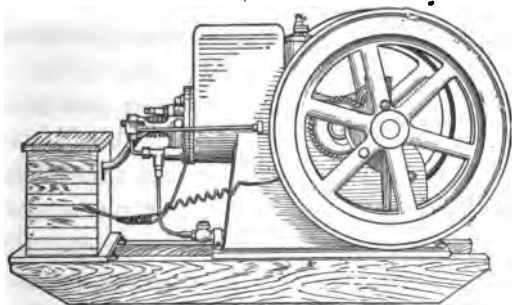
FIG. 164.—A four-cycle gas engine.
