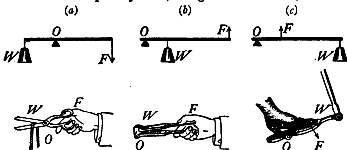
FIG. 86.—The three classes of levers.
