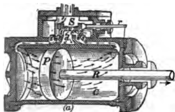
FIG. 158.—Cross-section view of cylinder and steam chest of a steam engine.
