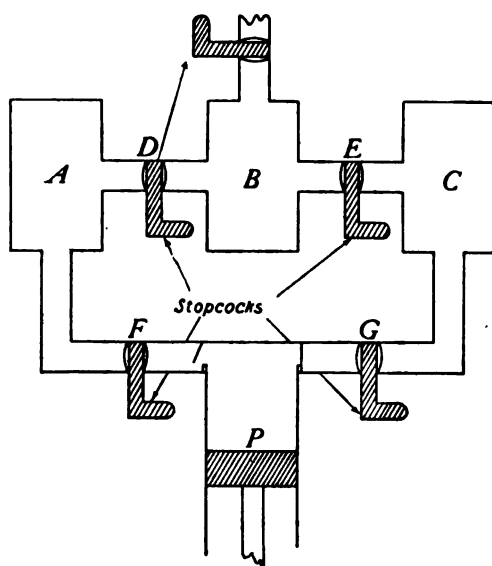
FIG. 207.—Air pressure apparatus to illustrate electrical pressure.
