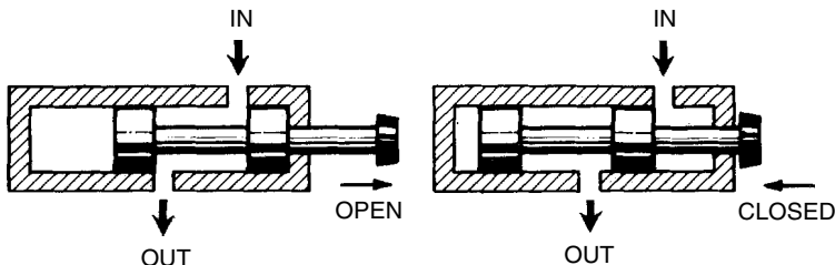
Figure 13.10 Two-way, fluid-power valve.
