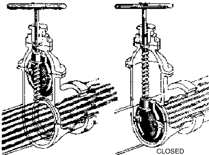
Figure 13.2 Non-rising-stem gate valve.
