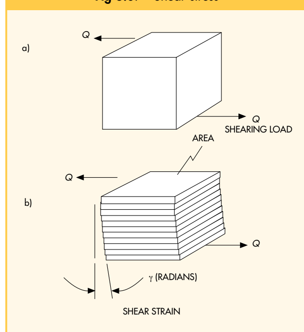
Fig 3.07 • Shear stress
