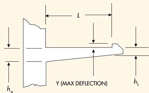
DYNAMIC STRAIN
