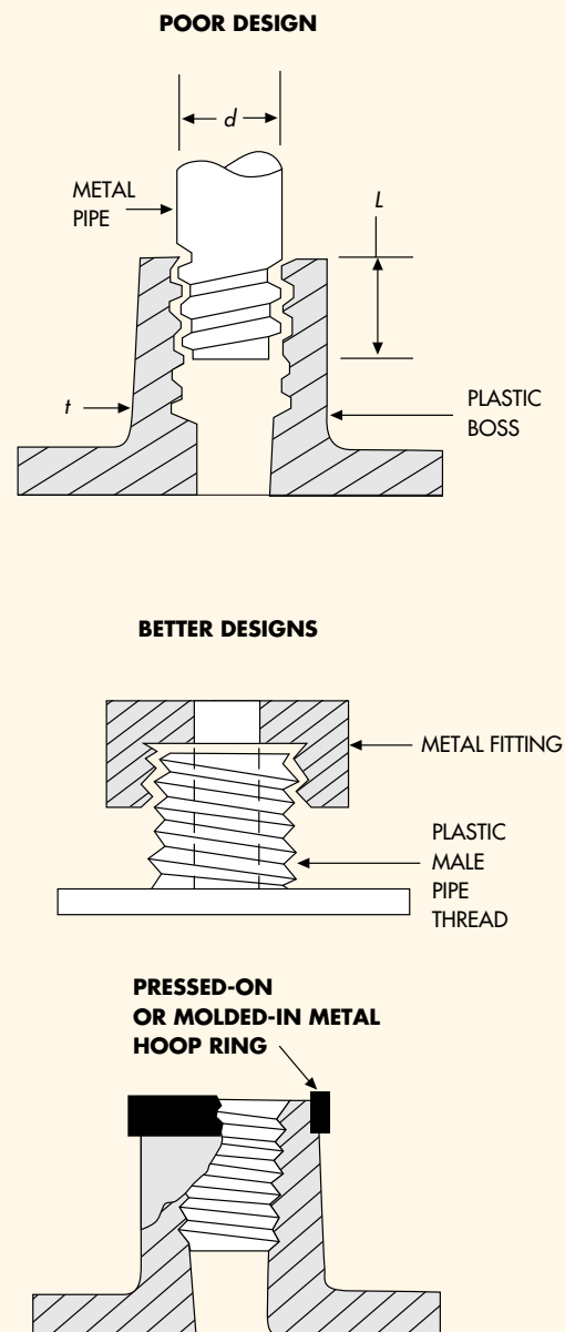
Fig 7.13 • Designing with pipe threads
