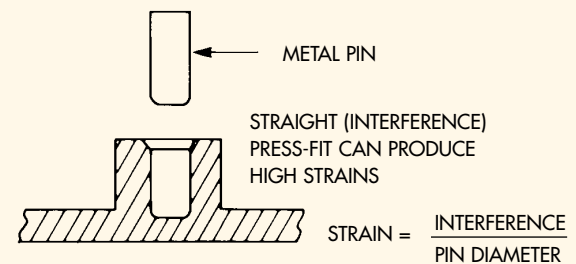
Fig 9.05 • Alternative press-fit designs for metal pins in plastic hub
