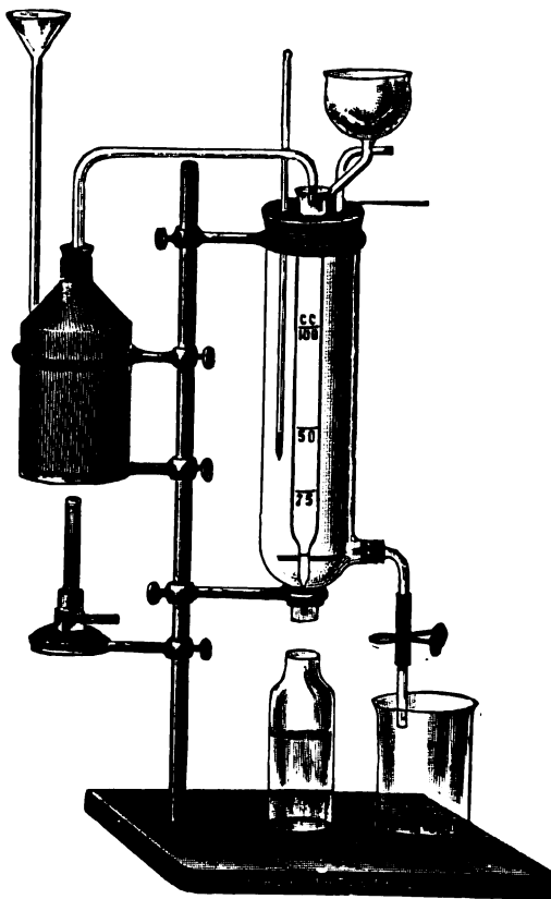
FIG. 46.—Archbutt's Viscometer.
