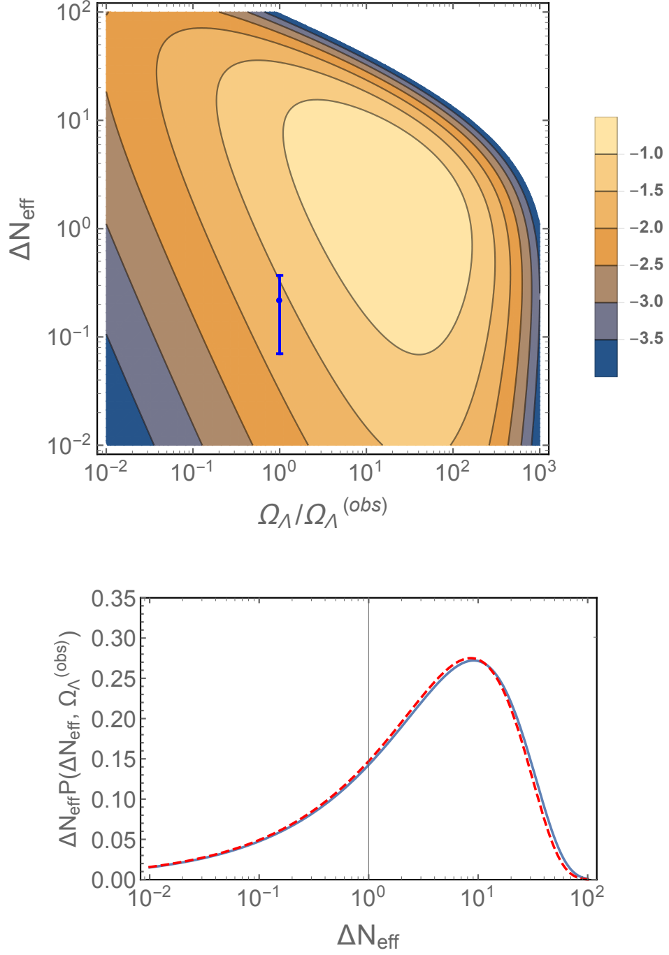
Figure 3. Same as Fig. 1 but with P_{\text{prior}} \propto 1/\sqrt{\Delta N_{\text{eff}}} .
