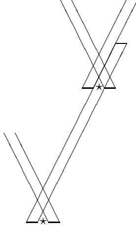
FIGURE 1. Picture of the block construction. Stars mark points of the renormalized lattice. When a parallelogram has an open path we declare the corresponding edge open.
