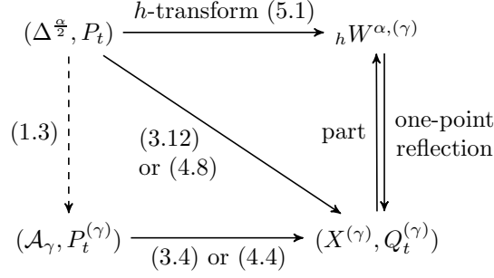
FIGURE 1. Globular or critical state under h -transform
