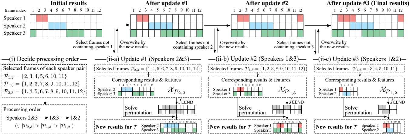
Fig. 1: The flow of the proposed method when the number of speakers is three. Given initial diarization results (top left), our method (i) picks up a pair of speakers iteratively in decreasing order of the number of frames and (ii) refines the diarization results of the two speakers using an end-to-end speaker diarization model.
