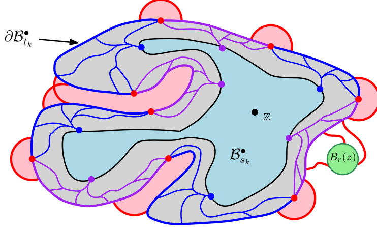
Figure 5: Illustration of the proof of Proposition 4.12. The points in the set \text{EndPts}_k of endpoints of arcs in \mathcal{I}_k are shown in red. We first use Theorem 2.16 to bound \#\text{EndPts}_k = \#\text{Conf}_k . Lemma 4.14 allows us to choose for each y \in \text{EndPts}_k a point z_y \in \partial \mathcal{B}_{t_k}^{\bullet} (not shown) such that an arc of B_{16\varepsilon^{\kappa_{\mathbb{R}}}}(z_y) disconnects the set \mathcal{C}_y^{\varepsilon^{\kappa_{\mathbb{R}}}} (defined just after Lemma 4.14) from \infty in \mathbb{C} \setminus \mathcal{B}_{t_k}^{\bullet} . The set which this arc disconnects from \infty , which contains \mathcal{C}_y^{\varepsilon^{\kappa_{\mathbb{R}}}} , is shown in pink. Note that the sets \mathcal{C}_y^{\varepsilon^{\kappa_{\mathbb{R}}}} for different choices of y are allowed to overlap. Lemma 2.14 and a union bound over y \in \text{EndPts}_k shows that with high probability, for each y \in \text{EndPts}_k , no D_h -geodesic from z to \partial \mathcal{B}_{s_{k+1}}^{\bullet} can enter any of the \mathcal{C}_y^{\varepsilon^{\kappa_{\mathbb{R}}}} 's. This together with Lemma 4.13 allows us to show that \text{Stab}_{k,r}(z) occurs for each (z, r) \in \mathcal{Z}_k such that P \cap B_r(z) \neq \emptyset . One such ball B_r(z) is shown in green and several segments of D_h(\cdot, \cdot; \mathbb{C} \setminus \overline{B_r(z)}) -geodesics from z to points of \partial B_r(z) are shown in red.
