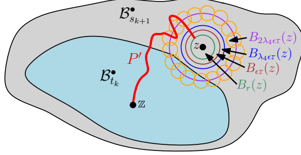
Figure 8: Illustration of the statement and proof of Lemma 4.22. In order to upper-bound \sup_{u \in \partial B_{2\lambda_4 \epsilon r}(z)} D_h(z, u; \mathcal{B}_{s_{k+1}}^{\bullet} \setminus \overline{B_{\epsilon r}(z)}) , we cover \partial B_{2\lambda_4 \epsilon r}(z) by Euclidean balls of radius \epsilon r/2 (orange) and upper-bound the D_h -diameters of these balls using condition 3 (Hölder continuity) in the definition of \mathcal{E}_{\mathbb{R}} . Each of these balls is disjoint from B_{\epsilon r}(z) and is contained in \mathcal{B}_{s_{k+1}}^{\bullet} , which leads to (4.61). Using Lemma 4.22 we get an upper bound for the D_h -length of the segment of a D_h(\cdot, \cdot; \mathbb{C} \setminus \overline{B_r(z)}) -geodesic from z to a point of \partial B_r(z) (such as the one shown in red) stopped at the last time it hits \partial B_{2\lambda_4 \epsilon r}(z) . This upper bound allows us to prevent such a D_h -geodesic from exiting \mathcal{B}_{s_{k+1}}^{\bullet} . These considerations lead to the proofs of Lemmas 4.16 and 4.19.
