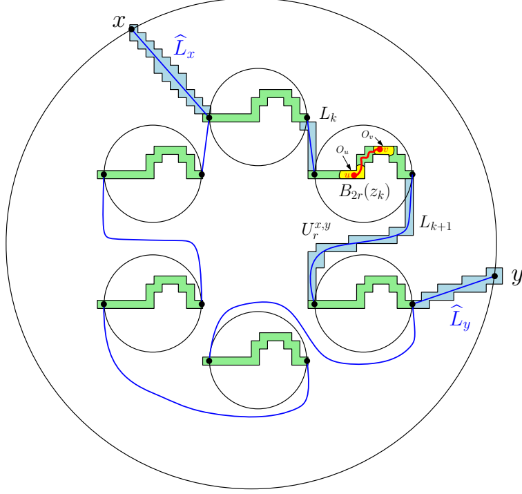
Figure 11: Illustration of the statement and proof of Lemma 5.8. To get an event with probability close to 1, instead of just an event with uniformly positive probability, we consider a large number of disjoint balls B_{\rho r}(z) centered at a finite set of points \mathcal{Z} \subset \partial B_r(0) and use Lemma 2.7 to argue that with high probability, the event F_{\rho r}(z) of Lemma 5.6 occurs for a suitably “dense” set of points z \in \mathcal{Z} . Then, we link up the tubes V_{\rho r}(z) for z \in \mathcal{Z} (light green) via deterministic paths L_k (blue). For a given choice of points x, y \in \partial B_{2r}(0) with |x - y| \geq \delta r , we define U_r^{x,y} to be the union of the sets V_{\rho r}(z) for points z \in \mathcal{Z} along the counterclockwise arc of \partial B_r(0) from x/2 to y/2 , the squares of \mathcal{S}_{\varepsilon_1 \rho r}(B_r(0)) which intersect the deterministic paths joining these sets V_{\rho r}(z) , and paths of squares starting from each of x and y (light blue). The sets O_u and O_v from assertion 2 are shown in yellow.
