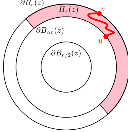
Figure 9: Illustration of the statement of Lemma 5.5. The lemma asserts that with probability at least p_0/8 , there is a D_h -geodesic (red) between points u and v in the inner and outer boundaries, resp., of the pink half-annulus H_r(z) which is contained in \overline{H_r(z)} and satisfies \tilde{D}_h(u, v) \leq c'_1 D_h(u, v) . The main task of Section 5 is to force a D_h -geodesic between two far away points to get near a \tilde{D}_h -geodesic like the red one in the picture.
