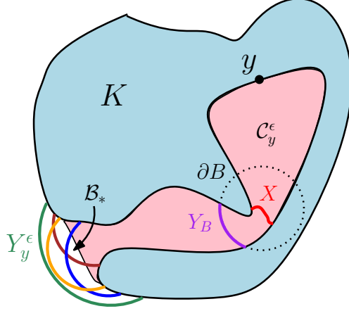
Figure 7: Illustration of the proof of Lemma 4.14. The set \mathcal{C}_y^\varepsilon is shown in pink. We have shown the boundary of a (non-maximal) ball B \in \mathcal{B} as a dashed line and the associated arc Y_B \subset \partial B \setminus K in purple. Each set X as in the lemma statement is contained in such a ball B and lies in the bounded connected component U_B of \mathbb{C} \setminus (Y_B \cup K) . Several arcs Y_B for maximal balls B \in \mathcal{B}_* are shown in various colors. Any two such arcs must intersect each other, so the Euclidean diameter of their union is at most 8\varepsilon . The set Y_y^\varepsilon (green) in the lemma statement is chosen so as to disconnect this union from \infty in \mathbb{C} \setminus K .
