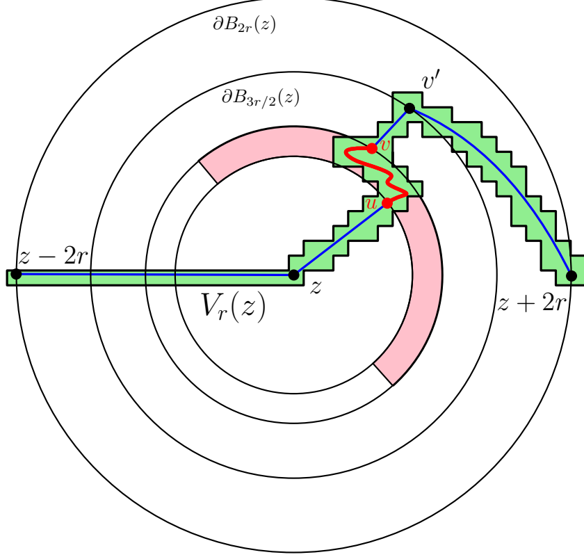
Figure 10: Illustration of the statement and proof of Lemma 5.6. Building on the setting of Figure 9, we show that there is a deterministic long narrow “tube” V_r(z) (light green), which is the interior of the set of \varepsilon_1 r \times \varepsilon_1 r squares with corners in \varepsilon_1 r \mathbb{Z}^2 which intersect a certain path from z - 2r to z + 2r , with the following property. With positive probability, every path in the tube from a point near z - 2r to a point near z + 2r has to get near a pair of points u, v in the tube for which \tilde{D}_h(u, v) \leq c'_1 D_h(u, v) . We will eventually add a bump function to h which takes a very negative value in such a tube in order to force a geodesic between points which are far away from B_{2r}(z) to get near u and v .
