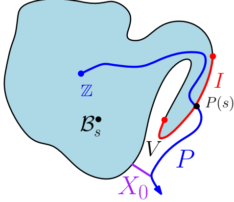
Figure 6: Illustration of the statement and proof of Lemma 4.13. If P gets d^{\mathbb{C} \setminus \mathcal{B}_s^\bullet} -close to \partial \mathcal{B}_s^\bullet \setminus I , then there is a set X_0 of small Euclidean diameter which intersects P and \partial \mathcal{B}_s^\bullet \setminus I . Moreover the Hölder continuity condition in the definition of \mathcal{E}_r implies that the Euclidean diameter of the segment of P between s and the first time it hits X_0 is small. The union X of this segment and X_0 disconnects one of the endpoints of I from \infty .
