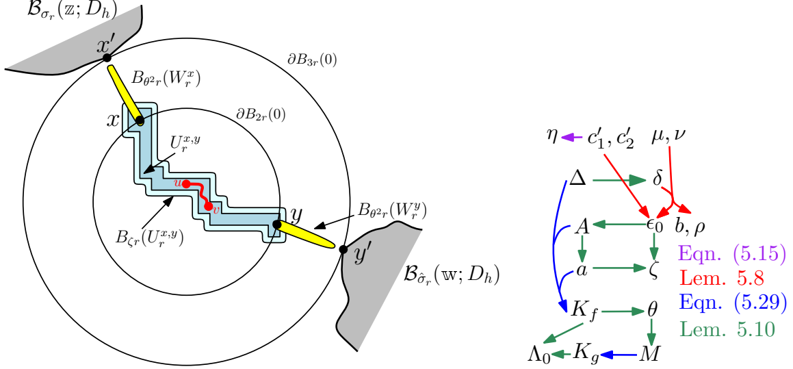
Figure 12: Left: Illustration of the definition of the event E_r . The blue set in the middle is the set U_r^{x,y} of Lemma 5.8. The light blue region surrounding it is B_{\zeta r}(U_r^{x,y}) , which is the support of the bump function f_r^{x,y} . The yellow regions are the supports of the bump functions g_r^x and g_r^y , which are used to force D_h -geodesics started from points outside of B_{3r}(0) to enter B_{\zeta r}(U_r^{x,y}) . The figure shows the relevant set for one pair of points x, y \in \partial B_{2r}(0) , but all of the conditions in the event E_r are required to hold simultaneously for all pairs of points x, y \in \partial B_{2r}(0) with |x - y| \geq \delta r . This is important since in Section 5.6 we will take x' = (3/2)x and y' = (3/2)y to be the random points where the metric balls based at the starting and ending points of a given geodesic (here shown in grey) first hit \partial B_{3r}(0) . Right: Schematic diagram of how the various quantities in the definitions of E_r and \mathcal{G}_r are chosen. An arrow between two parameters indicates that one is chosen in a way which depends directly on the other. The colors indicate where the choice is made. Most of the choices in the figure depend on \mathfrak{p} , but this is not illustrated. In the end, all of the parameters depend only on \mathfrak{p}, \mu, \nu (and the choice of metric).
