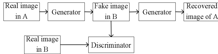
Fig. 3 Illustration of a one-way GAN in CycleGAN
