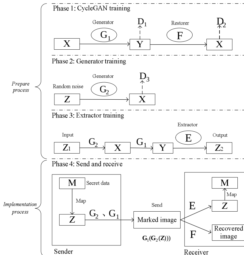
Fig. 4 Illustration of the proposed GRDH method
