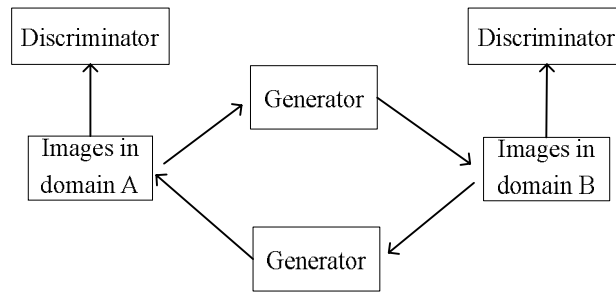
Fig. 2 Illustration of CycleGAN model
