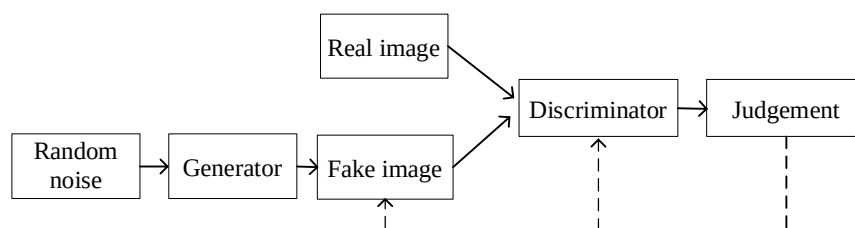
Fig. 1 Illustration of DCGAN model
