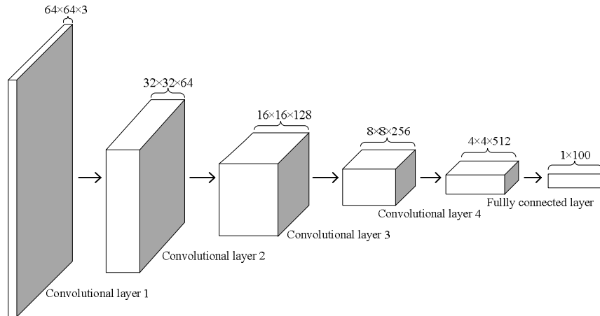
Fig. 5 Illustration of the extractor in GRDH method
