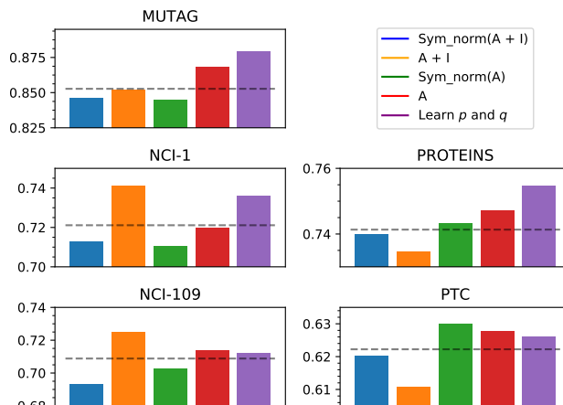
Figure 4: Each plot shows the mean classification accuracy for each message passing matrix of our search space, alongside the accuracy of PiNet when p and q are learned during training. The dashed lines indicate the mean accuracy of the manual search.
