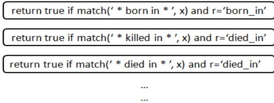
Figure 1: Rule Pattern Examples
