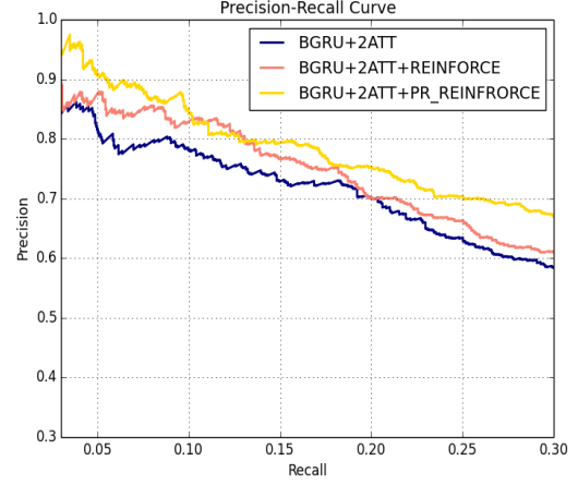
Figure 3: Precision/Recall Curves
