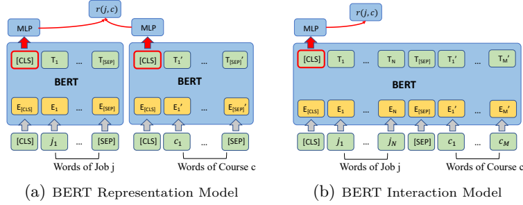
Fig. 3. BERT-based supervised text-only matching models.
