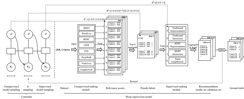
Fig. 1. Overview of the auto weak supervision model.
