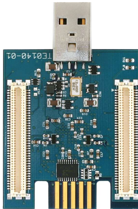
Figure 2: Micromodule Bottom Side
