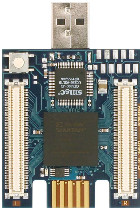
Figure 1: Micromodule Front Side
