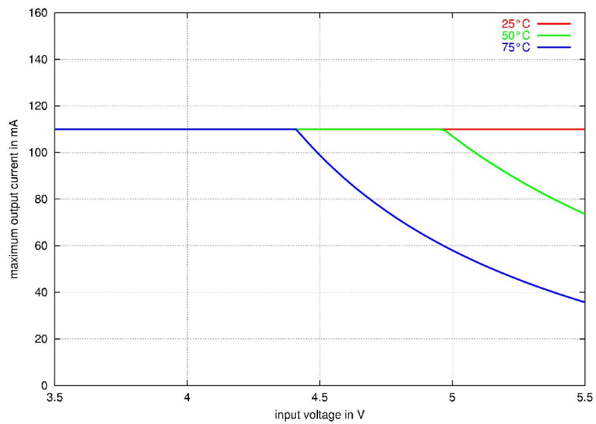
Figure 6: Available 3.3V power
